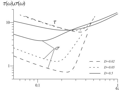
Fig. 5. The MST and its SD versus frequency for f(t) = A \sin(\omega t) (computer simulations) for three values of the noise intensity. Namely: D = 0.02 (long-dashed line), D = 0.05 (short-dashed line), D = 0.5 (solid line). The value of the bias current is i_0 = 0.5 , and the total current is i = 1.5 .
